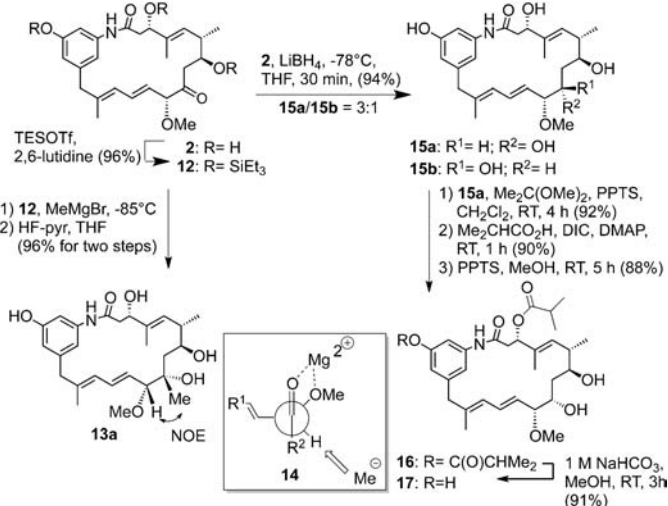
Scheme 4. Semisynthetic modifications of 2. A combined biosynthesis/semisynthesis approach using a late-stage mutant is shown. DIC = diisopropylcarbodiimide, DMAP = 4-dimethylamino pyridine, PPTS = pyridinium para -toluene hydrosulfonate, pyr = pyridine, TES = triethylsilyl, Tf = trifluoromethanesulfonyl, THF = tetrahydrofuran.
