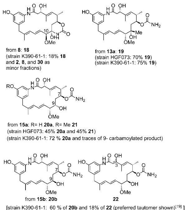
Figure 1. Preparation of the ansamitocin derivatives 18–22 after mutasynthetic derivatization of the modified proansamitocins 8 , 13a , and 15a,b . The compounds were prepared using a combined biosynthesis/mutasynthesis approach using a late-stage-blocked mutant followed by an early stage blocked mutant.
